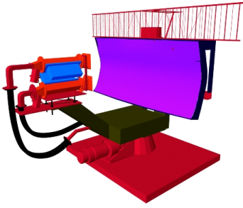
Airfield Surveillance Radar Dissectible (External): 10 Modeled
